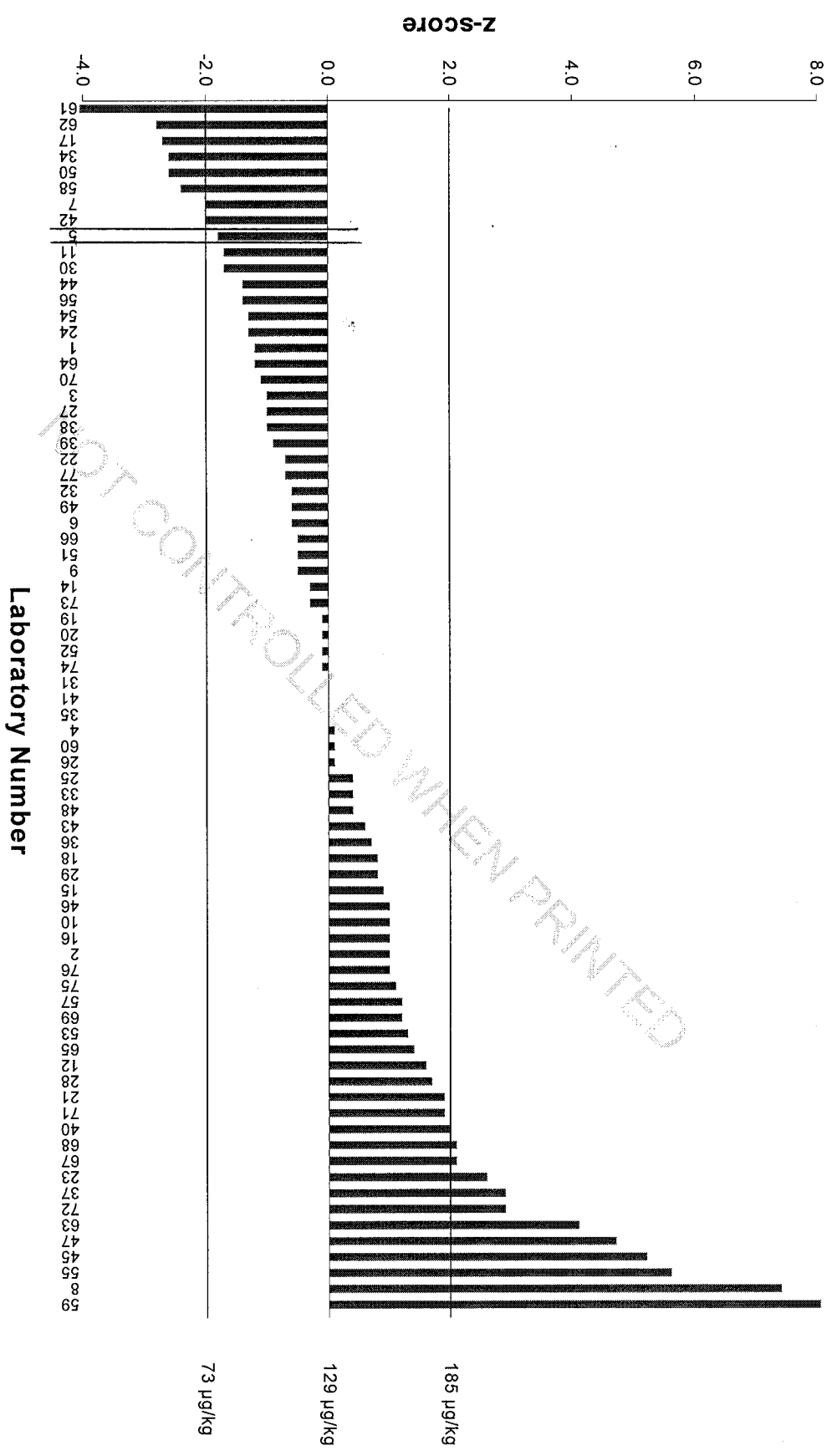
Figure 1: Z-Scores for ZON (129 µg/kg) in Animal Feed Test Material
